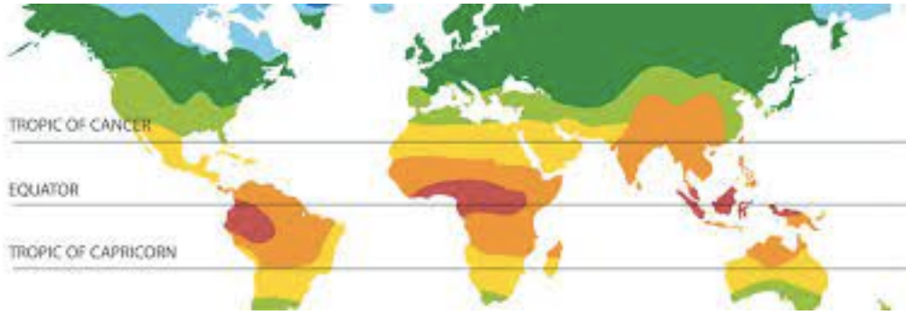
World Climate Zones
